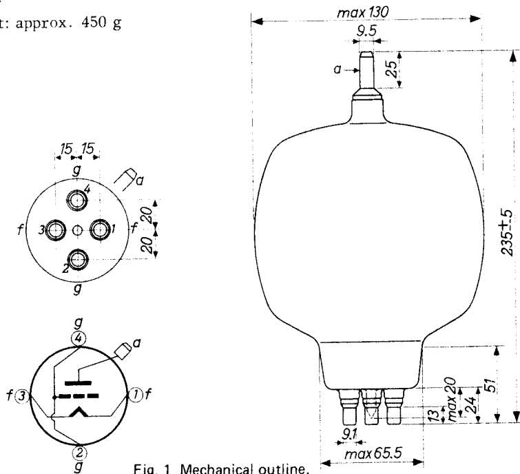
Fig. 1 Mechanical outline.
